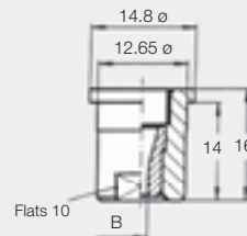
Series 548, weight: 13 g
