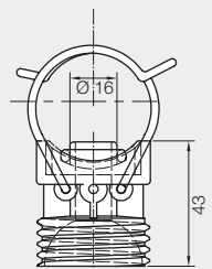
Double clamp
