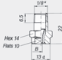
Series 550, weight: 13 g
