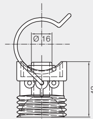
Single clamp
