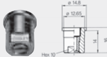
Series 652, Weight: 13 g
