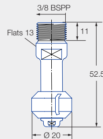
3/8 BSPP male thread
