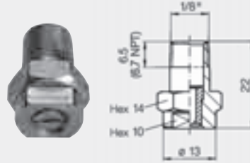
Series 608, Weight: 13 g
