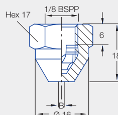
Series 214 Weight brass: 27 g
