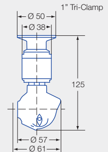
1" Tri-Clamp
