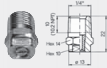
Series 602, Weight: 18 g
