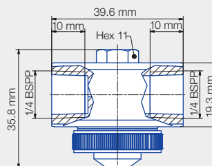
Weight brass: 200 g
