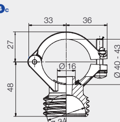
Eyelet clamp 1 1/4"
