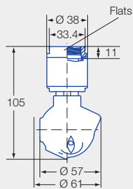
3/4 BSPP female thread
