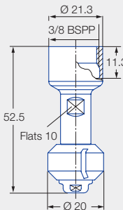
3/8 BSPP female thread
