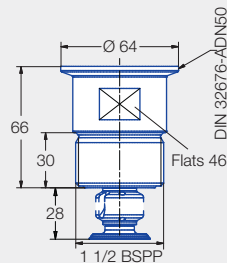
Male thread
