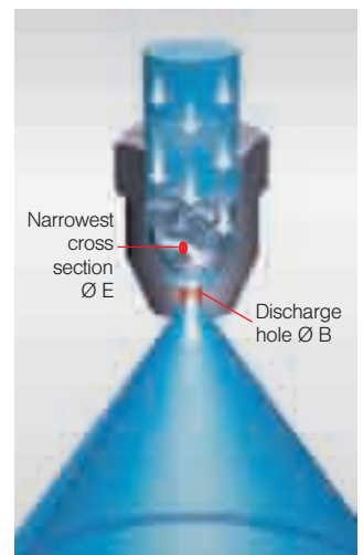
Figure 7: Narrowest cross section
