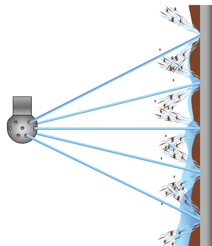
Figure 14: Cleaning with a spray ball
